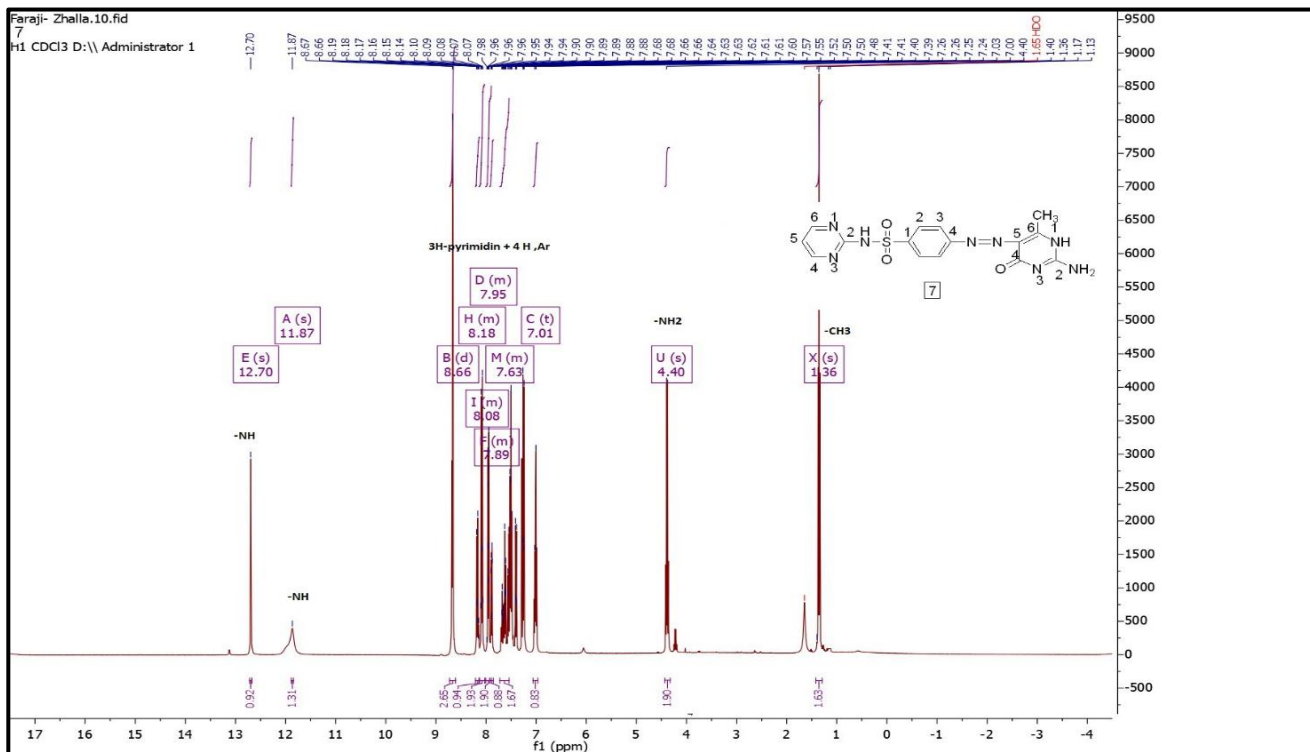
FIGURE 5: 1 H-NMR spectrum of 4-((2-amino-6-methyl-4-oxo-1,4-dihydropyrimidin-5-yl)diazenyl)-N-(pyrimidin-2-yl)benzenesulfonamide(7)
