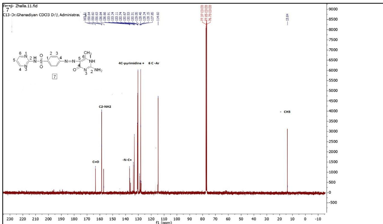
FIGURE 5: 1 H-NMR spectrum of 4-((2-amino-6-methyl-4-oxo-1,4-dihydropyrimidin-5-yl)diazenyl)-N-(pyrimidin-2-yl)benzenesulfonamide(7)
