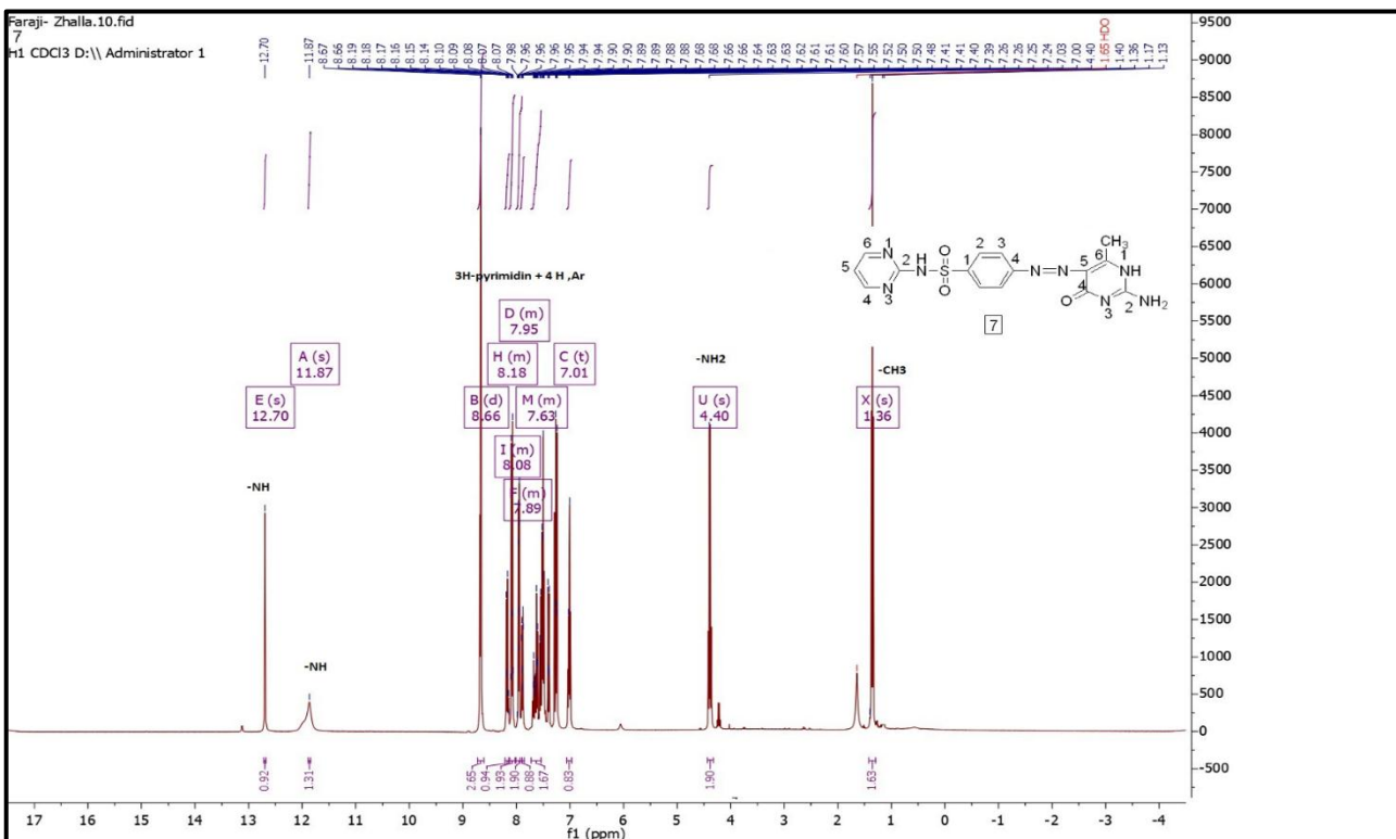
FIGURE 3: 13 C-NMR spectrum of 4-((1-benzoyl-5-methyl-3-oxo-2,3-dihydro-1H-pyrazol-4-yl)diazenyl)-N-(pyrimidin-2-yl)benzenesulfonamide (5)
