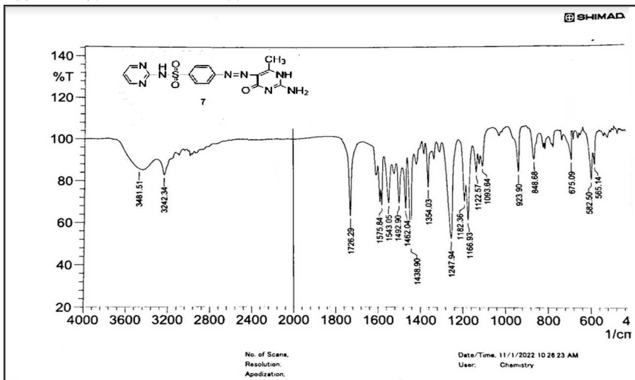
FIGURE 4: IR Spectrum of 4-((2-amino-6-methyl-4-oxo-1,4-dihydropyrimidin-5-yl)diazenyl)-N-(pyrimidin-2-yl)benzenesulfonamide(7)
