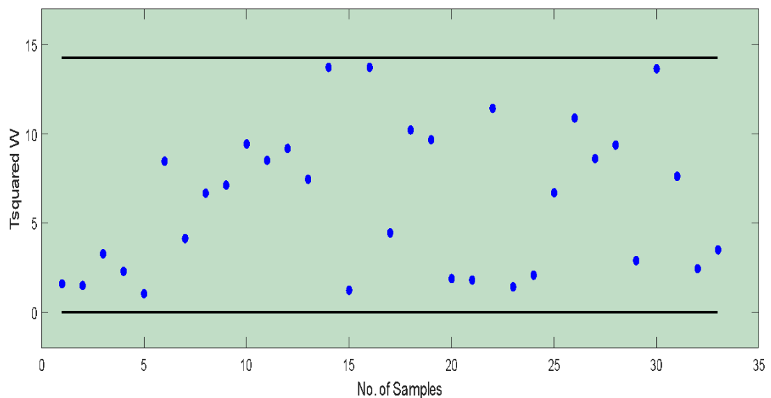
Fig. 9. Wavelet T^2 -Chart for real data.
